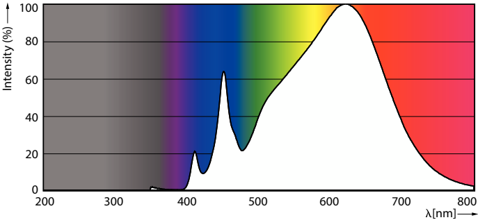
Spectral Power Distribution Colour - 10PAR30L/EXPERTCOLOR RETAIL/ F25/930/D
