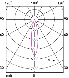
Light Distribution Diagram - 10PAR30L/EXPERTCOLOR RETAIL/F25/930/D
